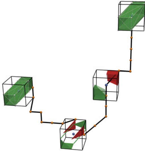
Figure 4: Gradient path tracing for computing arcs of extremum graph. Ascending 1-dimensional manifolds are computed for each 2-saddle. The gradient paths that constitute these ascending manifolds represent the arcs of the extremum graph. Note that they pass through regular points, entering and exiting its neighborhood via the lower and upper link, respectively.
