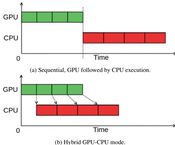
Figure 6: Hybrid GPU-CPU parallel computation for a dataset partitioned into 4 blocks. In the sequential execution model (a), point classification step (green) processes the blocks one by one on the GPU. Gradient path tracing (red) for the blocks executes on the CPU after point classification is complete for all blocks on the GPU. The CPU cores lie idle, waiting for the completion of critical point classification for all blocks on the GPU. In the hybrid GPU-CPU mode (b), gradient path tracing within the first block begins soon after it is processed by the GPU. The transfer of control from GPU to CPU for a block is indicated by arrows. The base of the arrow lies at the finishing time for a block on GPU and the tip lies at the time when that block is taken up for processing on the CPU.
