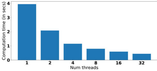
Figure 11: CPU scaling study for varying number of CPU threads. Experiments on the dataset Zeiss show good scaling up to 8 threads.
