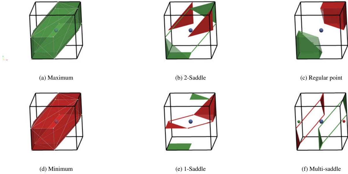
Figure 3: Critical points can be identified and classified based on the upper (red) and lower (green) link connectivity. The upper link of a maximum (a) is empty and the lower link is equivalent to a sphere, whereas the upper link of a minimum (d) is equivalent to a sphere and the lower link is empty. The upper link of a simple 2-saddle (b) consists of two connected components and its lower link consists of a single component, whereas the upper link of a 1-saddle (e) consists of a single component and the lower link consists of two connected components. Both the upper and lower links of a regular point (c) consist of a single component. The multi-saddle (f) is a degenerate structure that does exist in piecewise linear functions.
