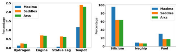
Figure 14: Statistics on the fraction of extremum graph nodes and arcs that survive post simplification. The number of surviving extrema, saddles, and arcs after applying the three simplification operations in sequence are shown as a fraction of the corresponding numbers in the unsimplified extremum graph.
