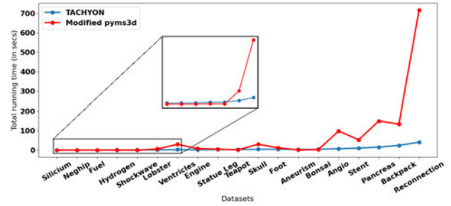
Figure 13: Runtime comparison between TACHYON and pyms3d [SN17]. TACHYON performs consistently better, often several orders of magnitude faster.
