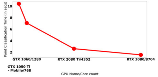
Figure 9: GPU scaling results.
